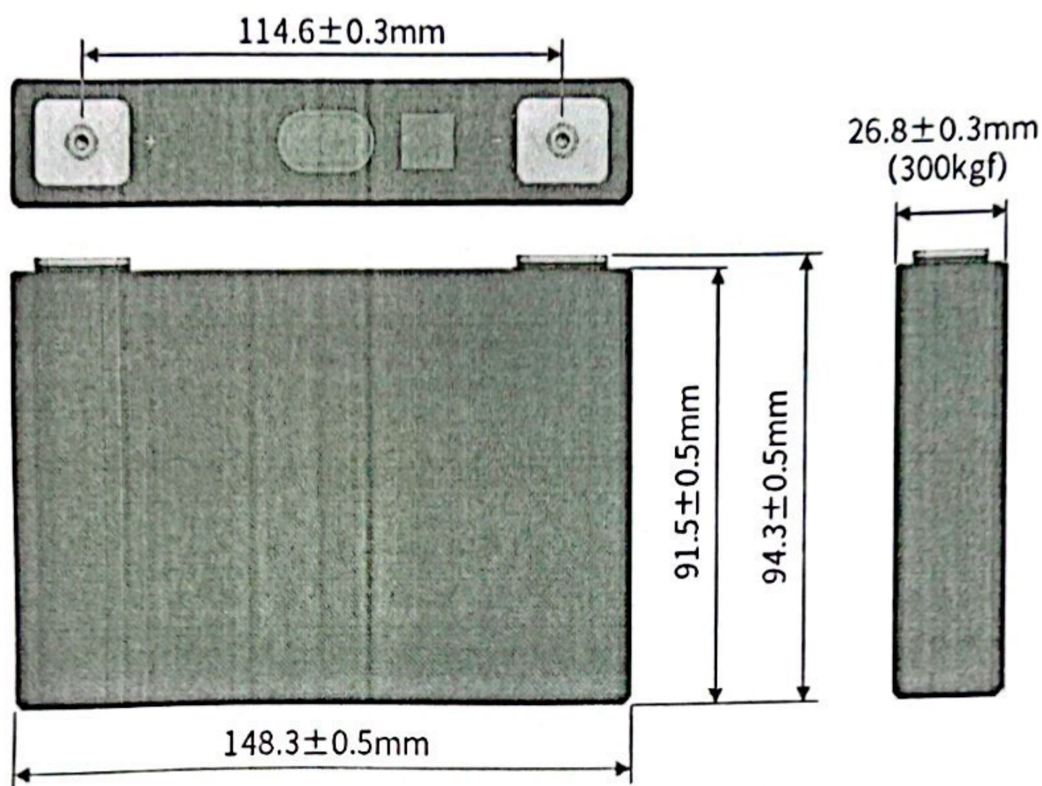
Fig.4 LF32 Battery Drawing 图 4 LF32 电池图纸
